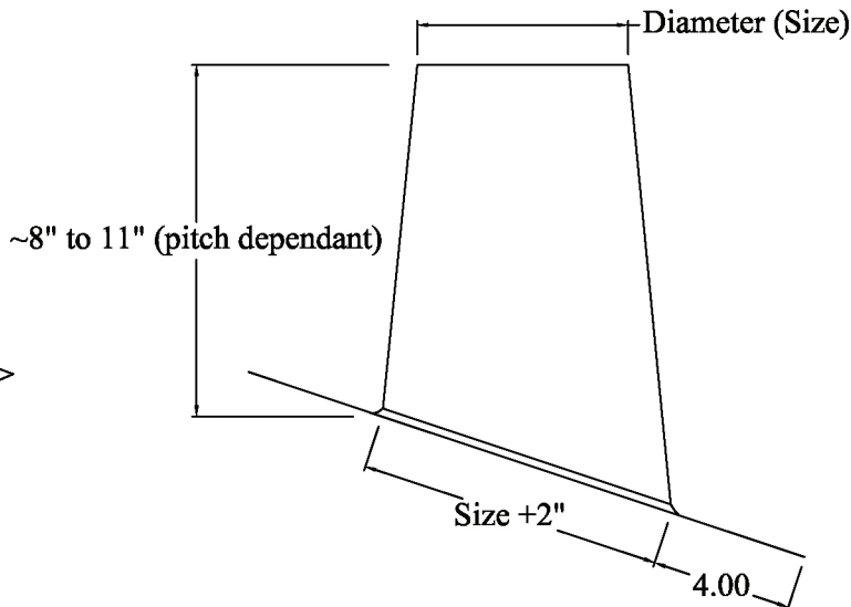
3/12 through 7/12 Pitch
